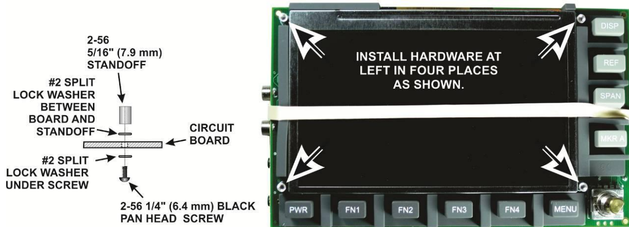
Figure 27. Mounting the Front Panel Standoffs.
