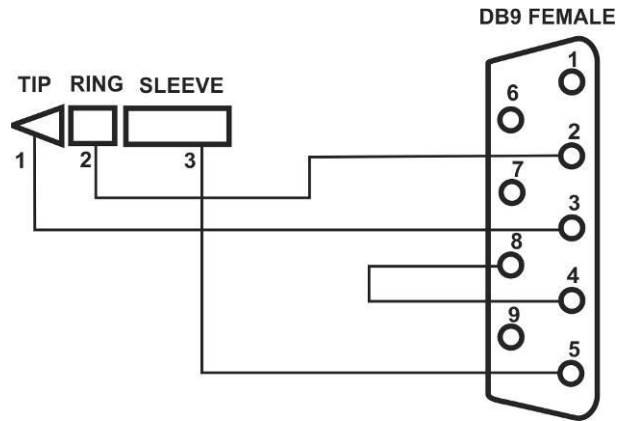
Figure 25. RS-232 Cable Schematic Diagram.
