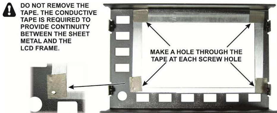
Figure 28. Front Panel Conductive Tape.
