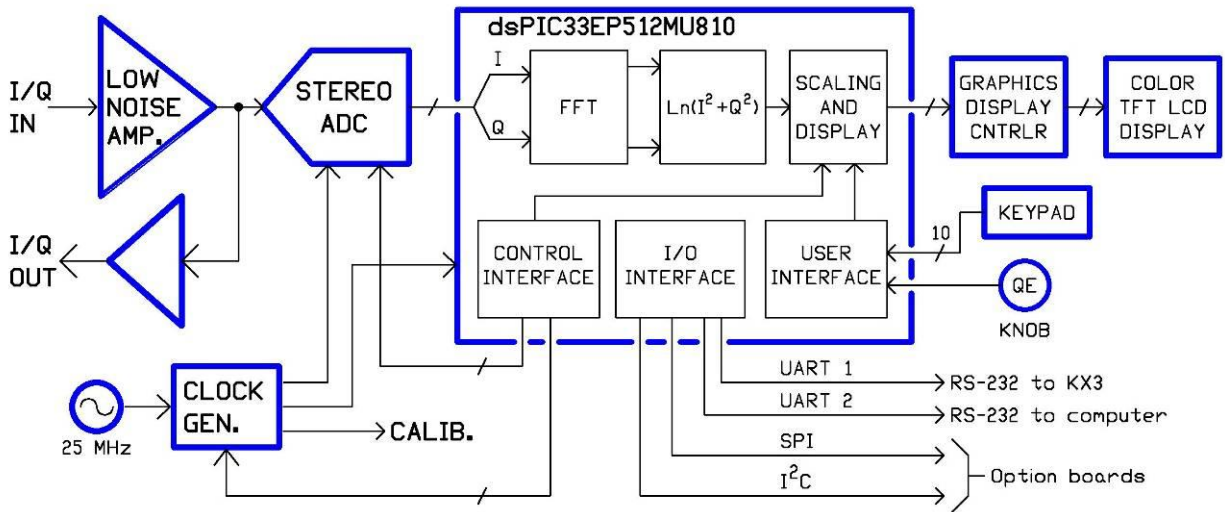
Figure 24. PX3 Simplified Block Diagram.
