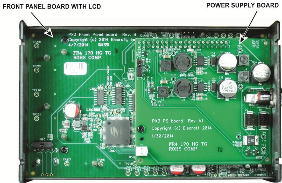
Figure 26 Assembled PX3 with Rear panel Removed.
