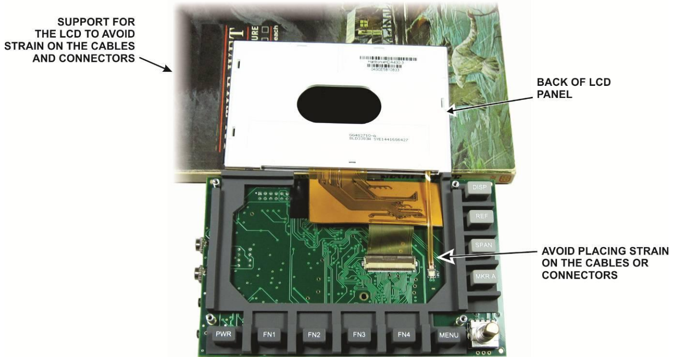
Figure 48. Removing LCD Panel from Rubber Key Matrix.
