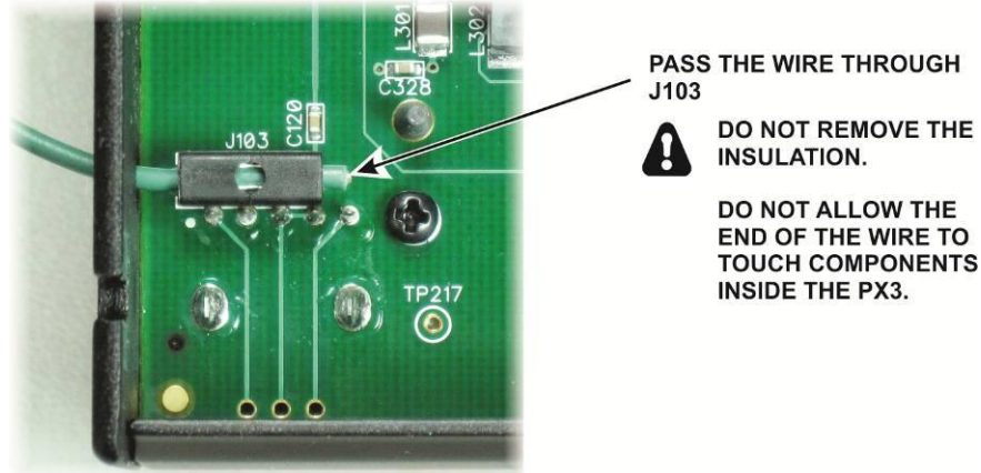
Figure 22. Calibrator Signal Pickup Wire Installed in the PX3.
