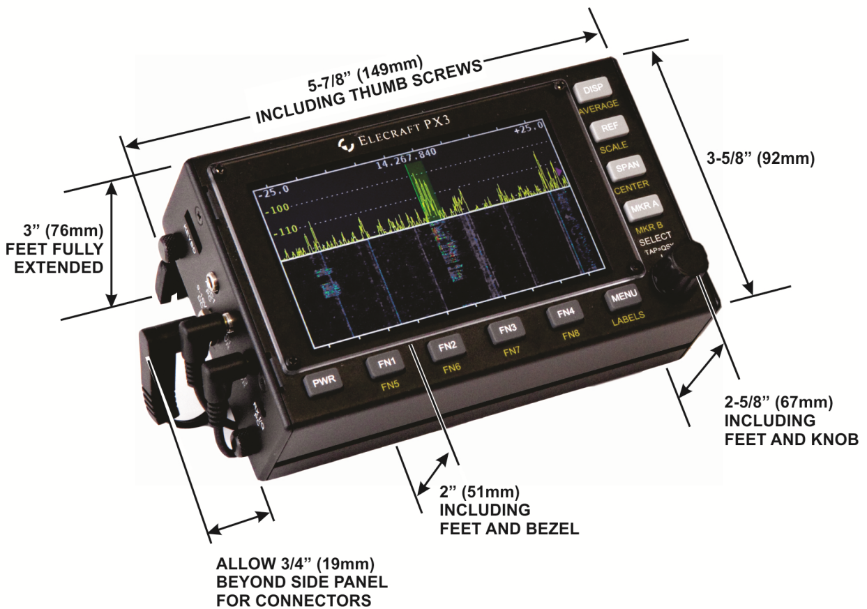
Figure 50. PX3 Dimensions.
