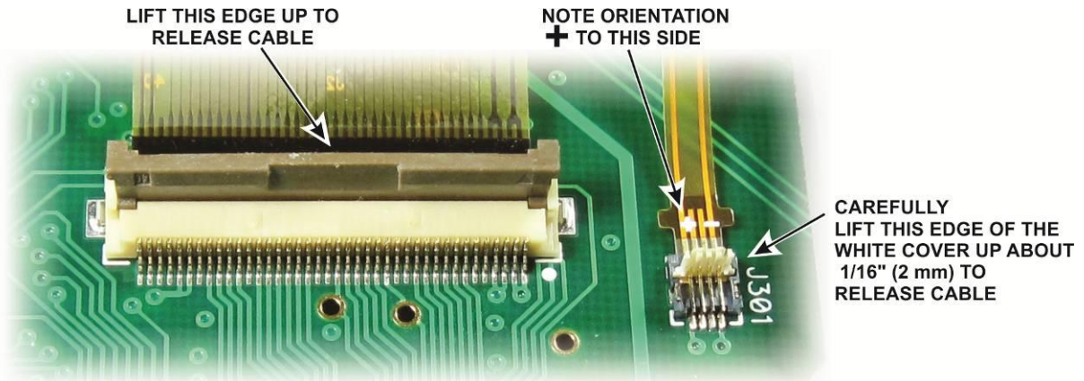
Figure 49. LCD Cable Connectors Opened.
