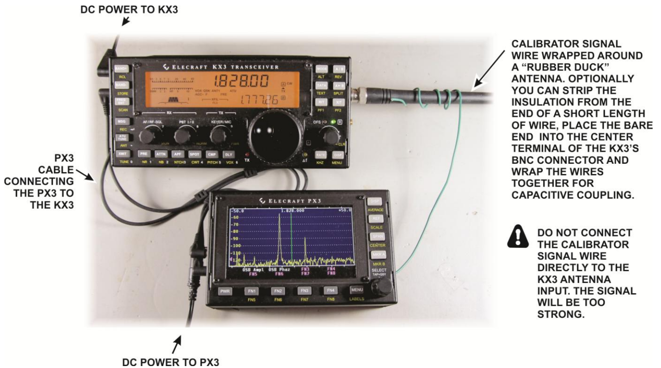
Figure 23. Opposite Sideband Nulling Setup Using Internal Signal Source.
