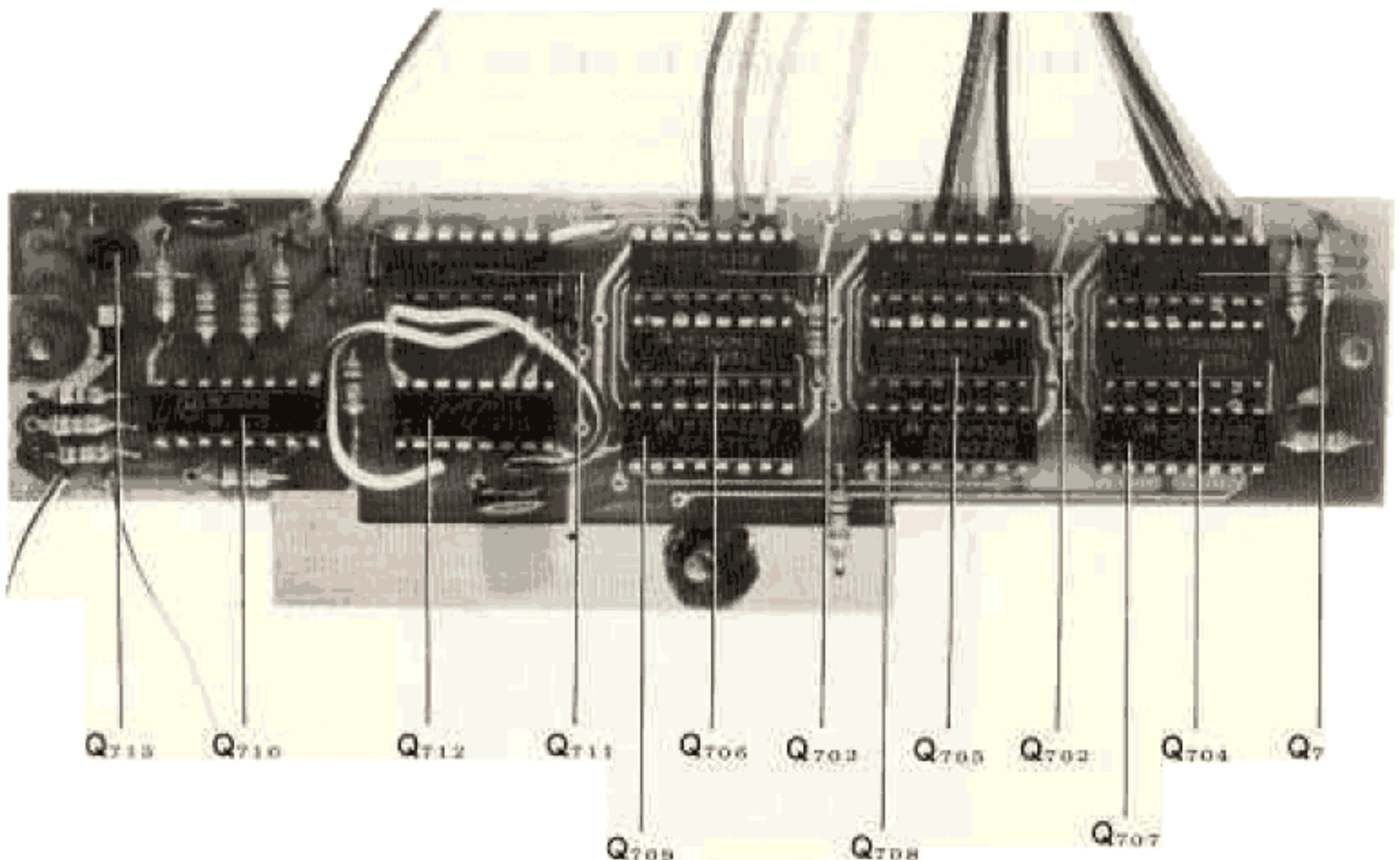
PLL CONTROL UNIT
