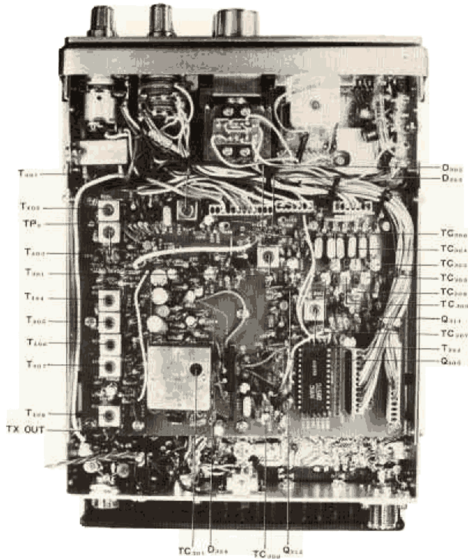
Figure 16 ALIGNMENT POINT
