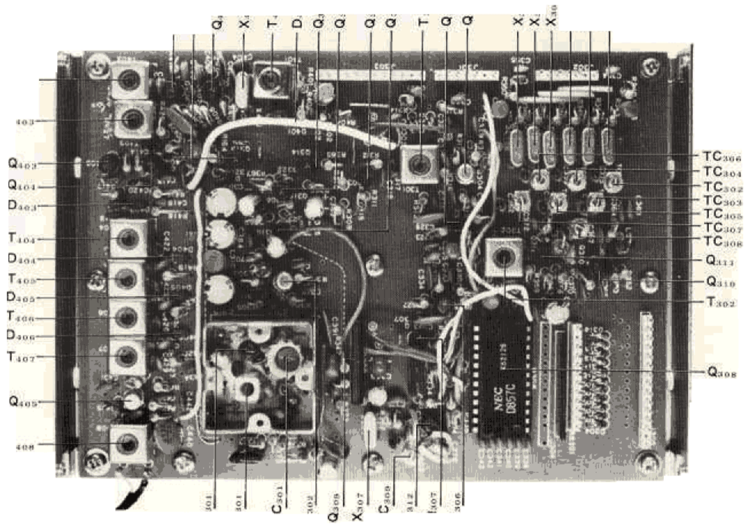
PLL
