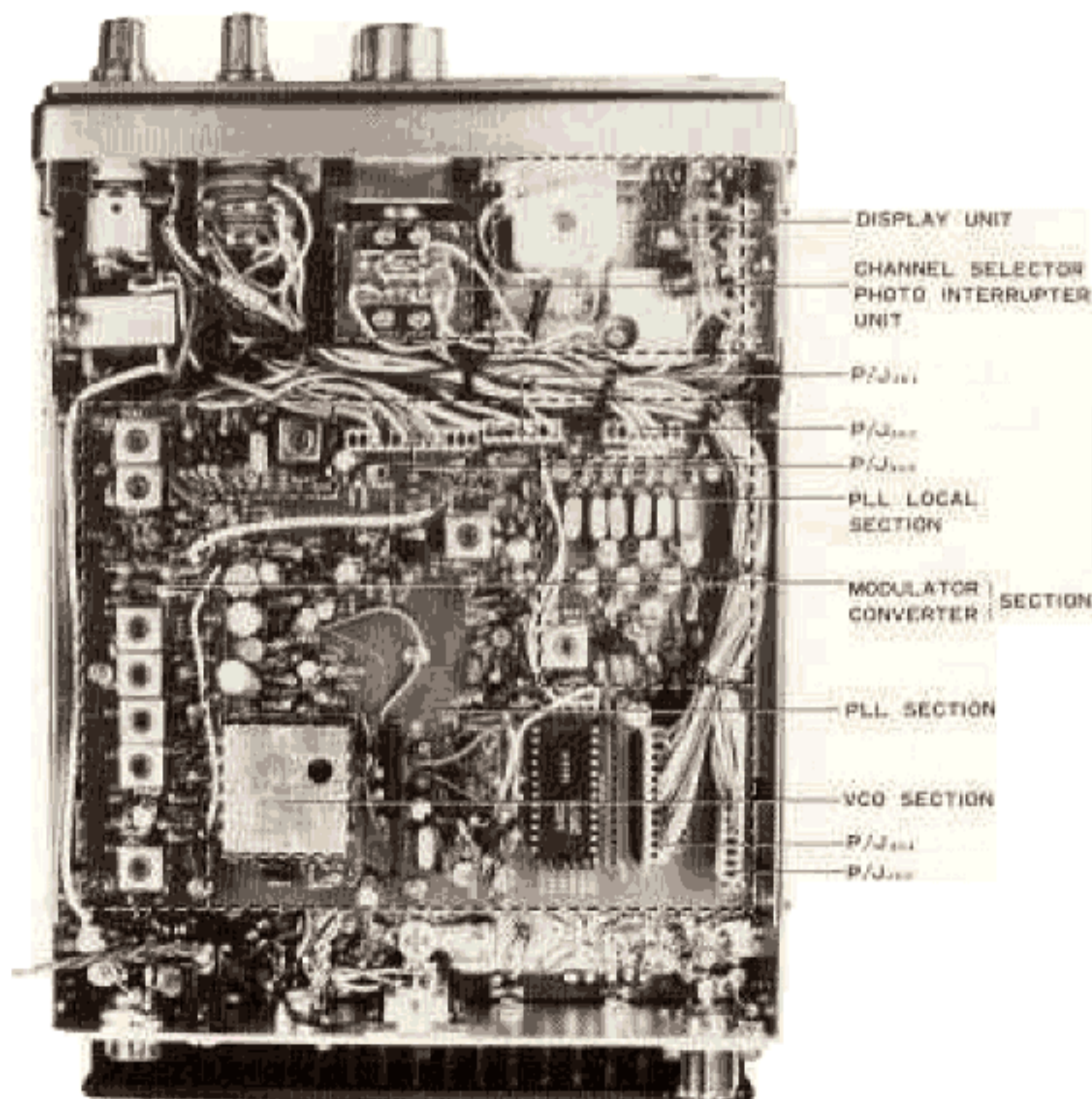
Figure 11 BOTTOM VIEW
