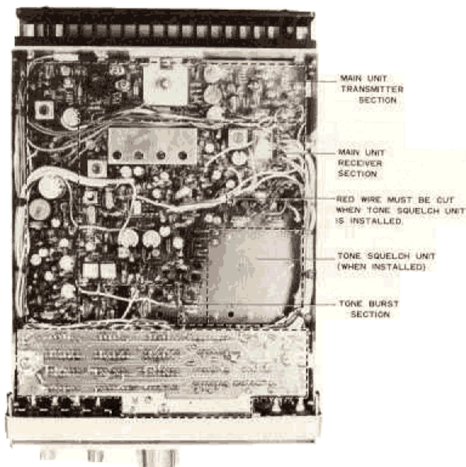
Figure 10 TOP VIEW
