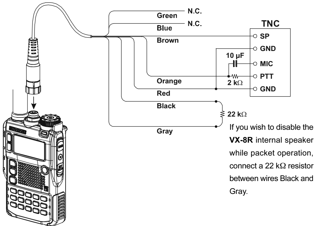
CT-M11 MIC/SP Connection Cable
