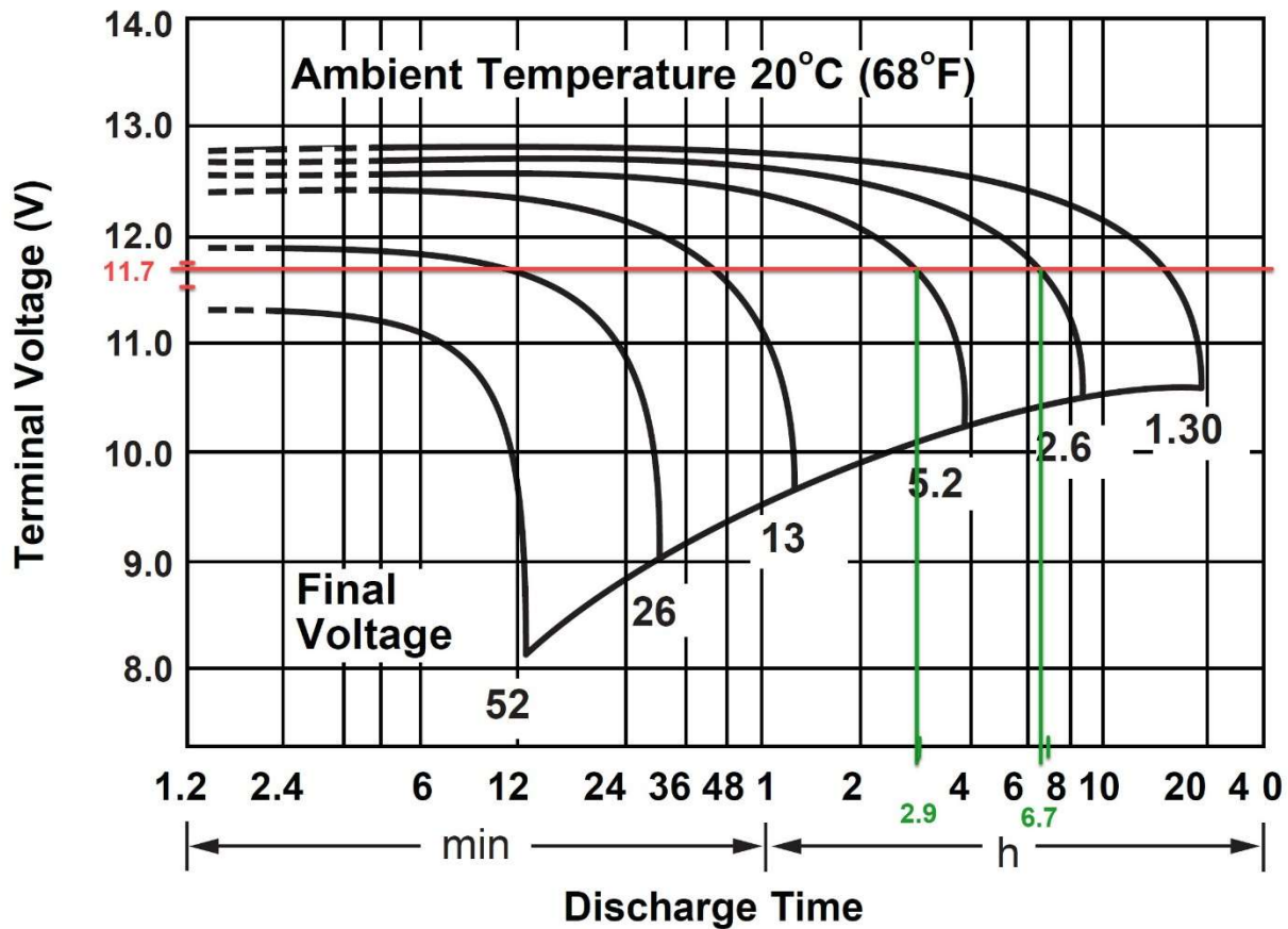
Figure 1: 12V 26Ah AGM Discharge Curves (Source: PowerSonic PS-12260 Datasheet, annotated)
