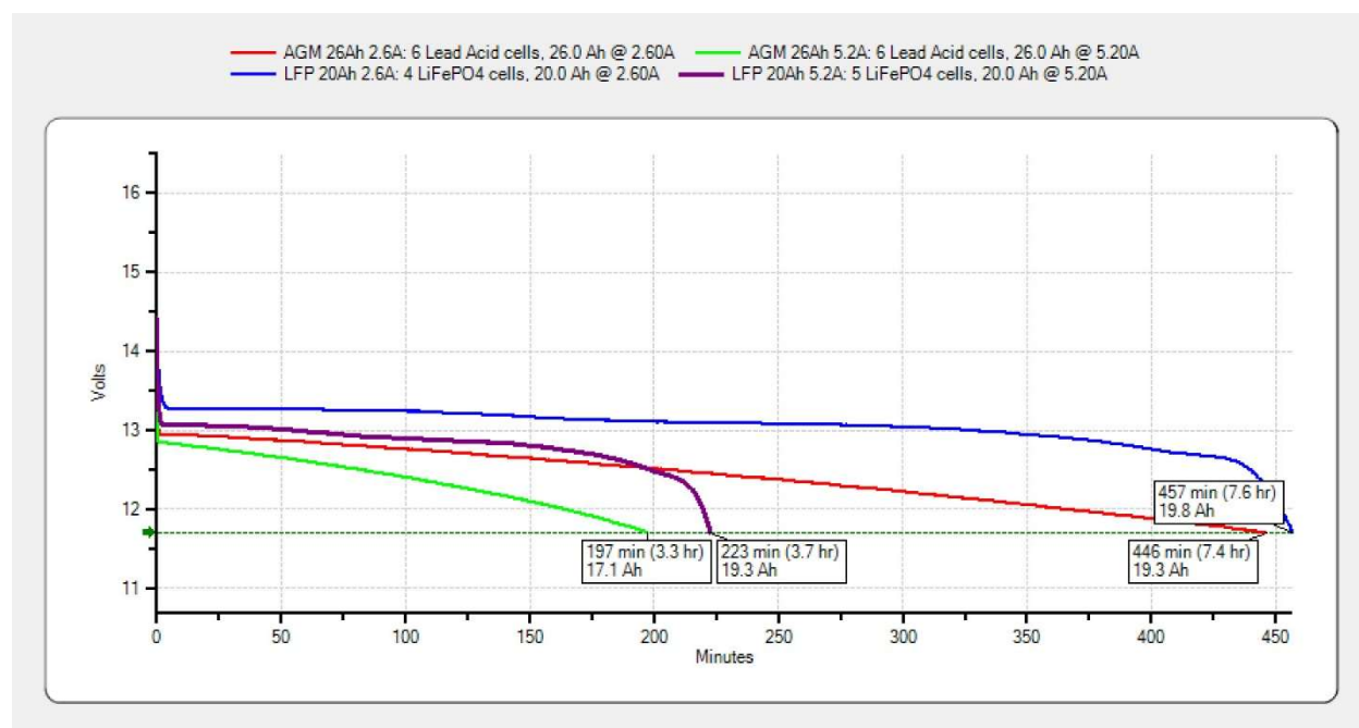
Figure 2: Test results for AGM and LFP Constant Current Discharge Tests at 2.6A and 5.2A
