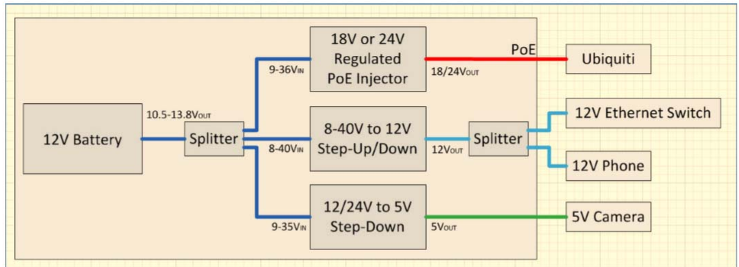
Ubiquiti Power Management
