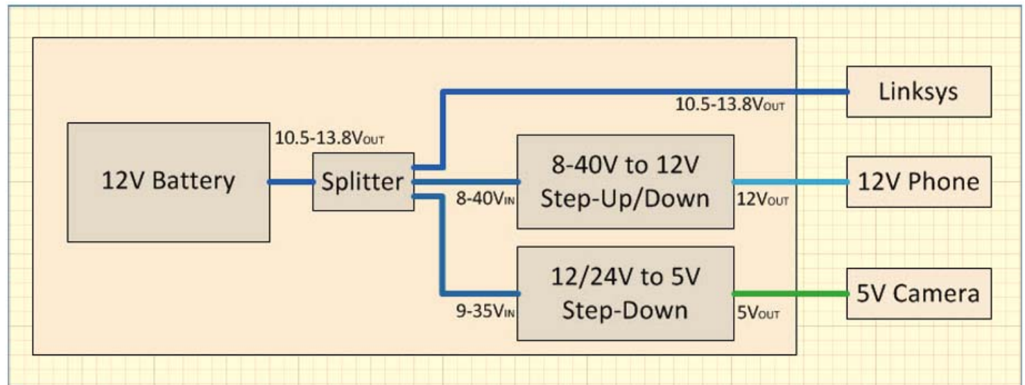
Linksys Power Management
