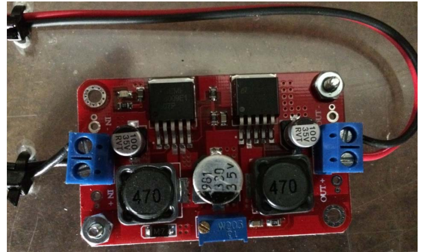
DC-DC Converter, 12vdc – variable
